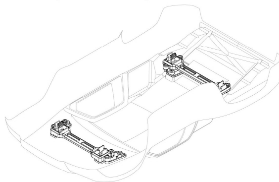
Completed Assembly (view from bottom)
