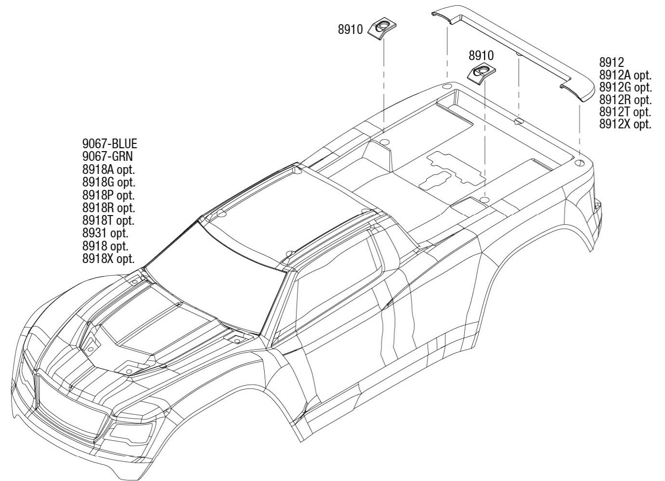
Completed Assembly (view from bottom)
