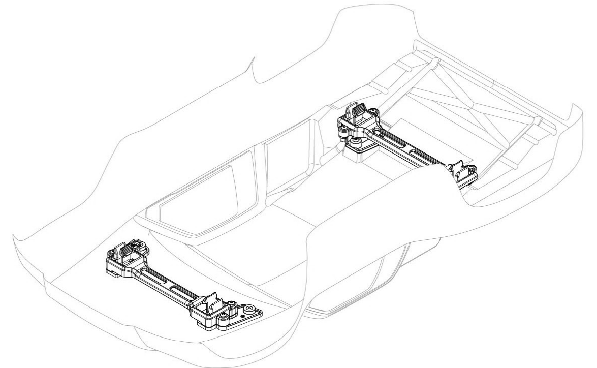
Completed Assembly (view from bottom)
